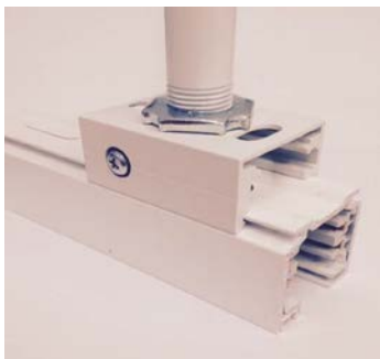
Threaded Rod secured to 198-00-0001-01 clip and track.
