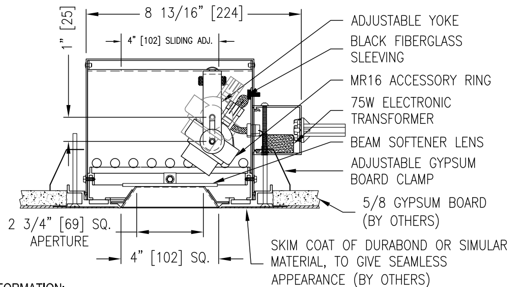
SECTIONED END VIEW
